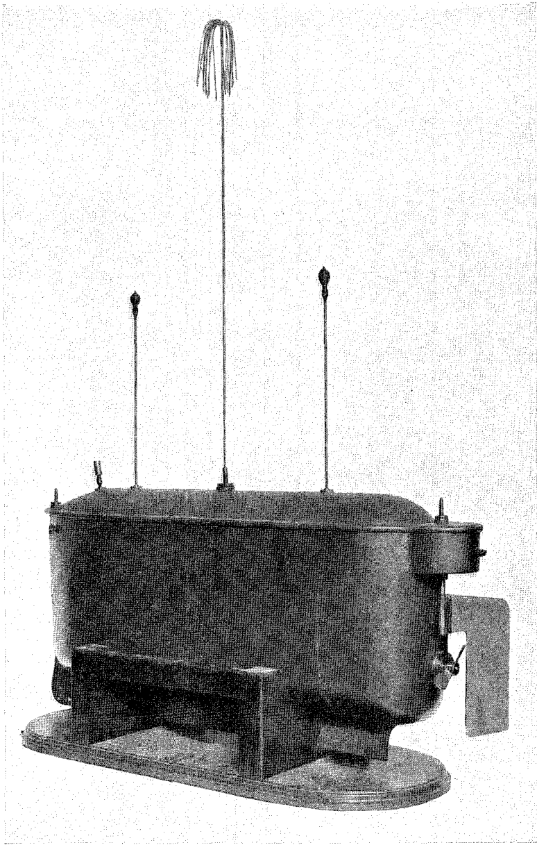
FIG. 2. THE FIRST PRACTICAL TELAUTOMATON.
